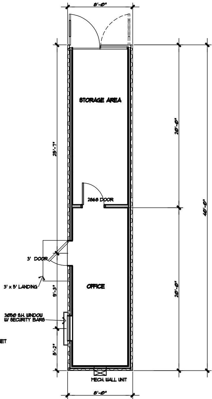
CONTAINER OFFICE FLOOR PLAN SCALE: 1/4" = 1'-0"
