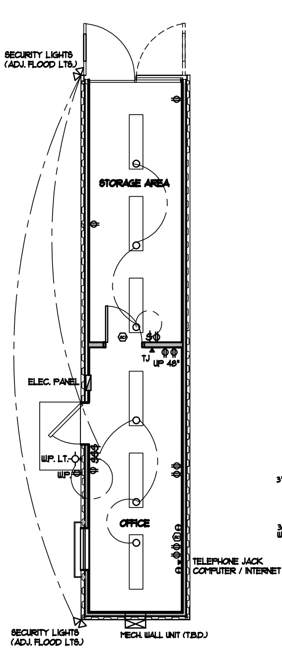
CONTAINER OFFICE POWER PLAN SCALE: 1/4" = 1'-0"
